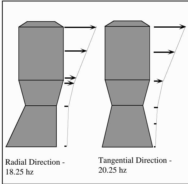
Figure 5: Operating deflection shapes of the swing motor.
